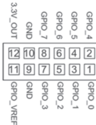
Figure 1-12: GPIO 2x6 Pin Assignments
