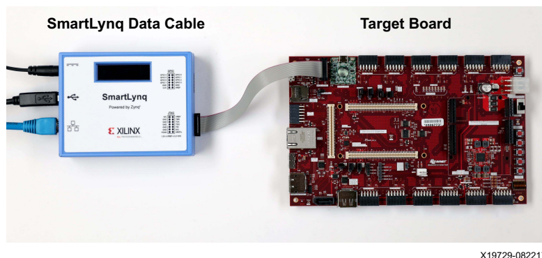
Figure 1-9: SmartLynq Data Cable JTAG Connection to the JTAG Interface on a Target Board
