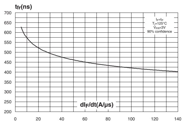
Figure 14: Forward recovery time versus di_F/dt (damper diode)
